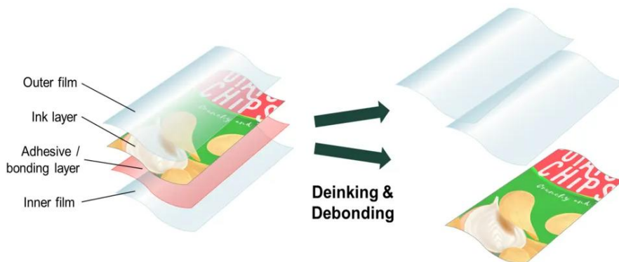
Illustration of the deinking and debonding process for recycling multilayer film packaging.
